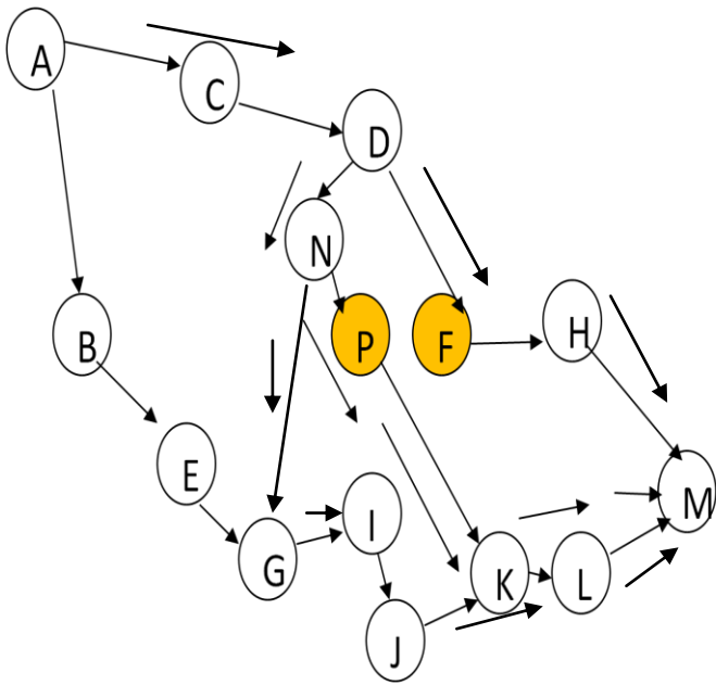
Figure 1. faulty Nodes and Apply Recovery Scheme
