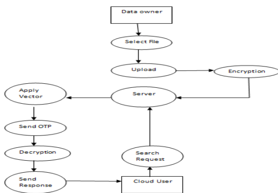
Fig.1 DataFlow Diagram
