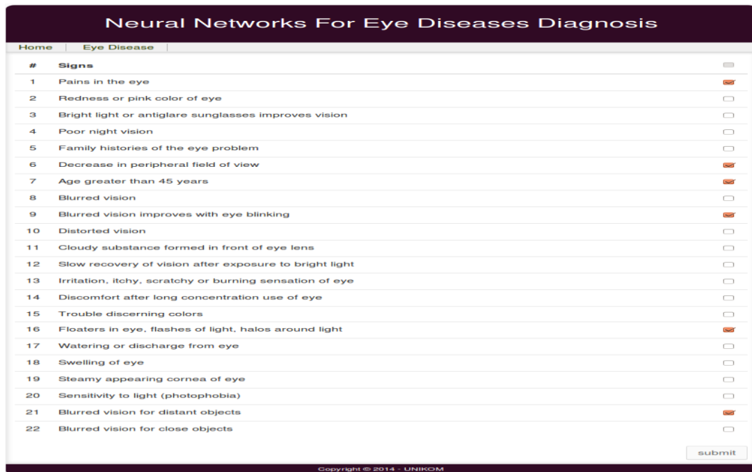
Fig. 1.- Select Symptom[3]
