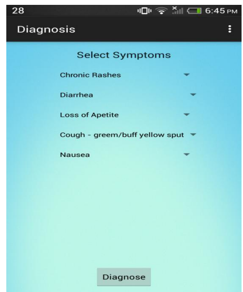
Fig. 5. - Select Symptoms
