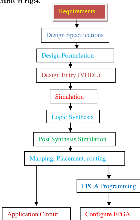
Fig:4 Digital System Design Flow Diagram
