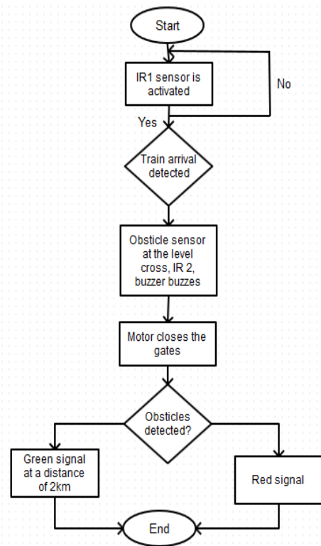
Fig. 3: Flowchart of opening of gate
