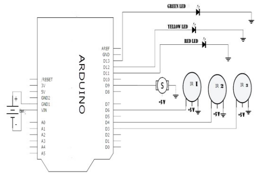
Fig. 10: Circuit diagram of the system
