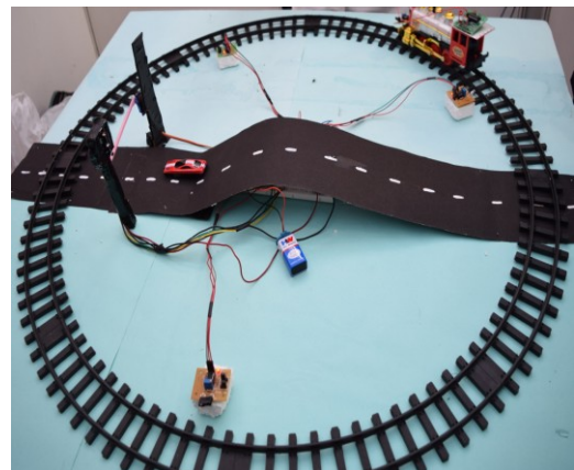
Fig. 12: Model of railway level cross
