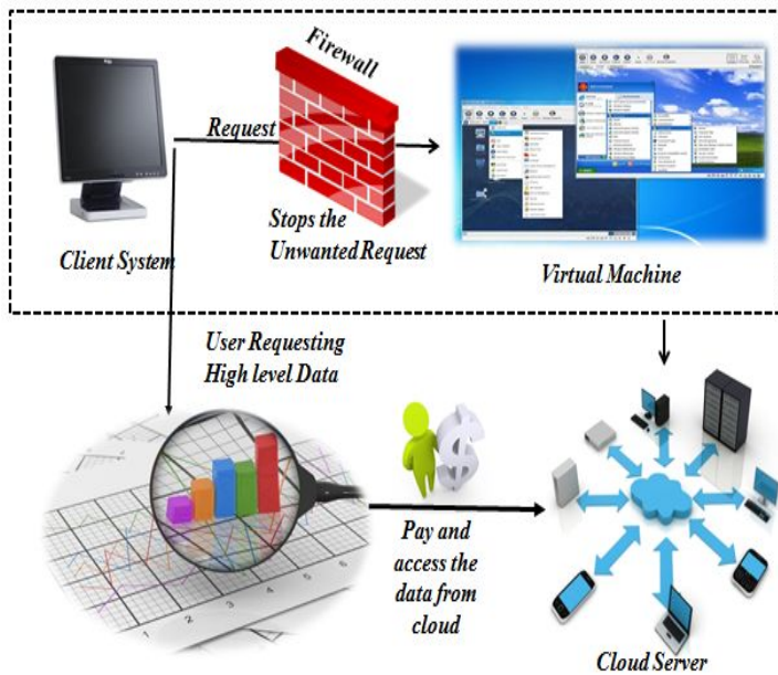
Fig 1. System Architecture
