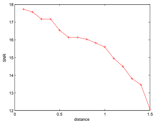
Fig.3.2 Plot showing the average SNR of QAM modulation techniques against distance for Sub-urban
