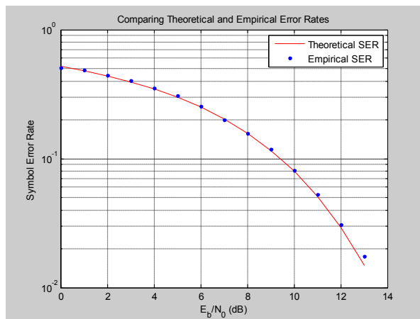
Fig.3.4 Plot showing the average Empirical Symbol error rate and Theoretical symbol error rate against SNR for the Environment under study.
