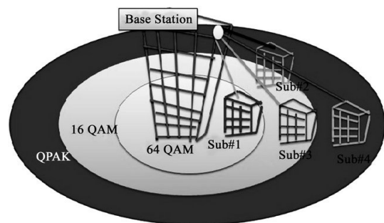
Fig 2.2 Adaptive Modulation
