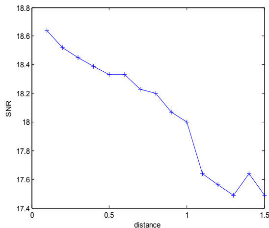
Fig.3.3 Plot showing the average SNR of QPSK modulation techniques against distance for Sub-urban
