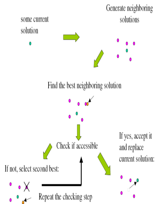
Fig 1 Basic structure of Tabu Search
